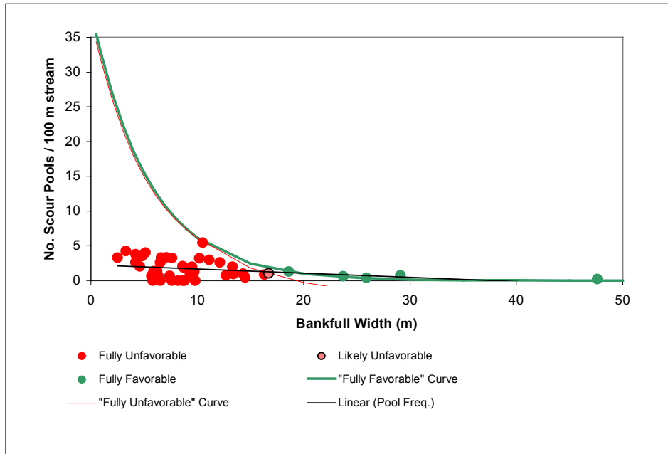
Figure 10. Pool frequency and EMDS interpretive curves as a function of bankfull width at 49 sample sites.
