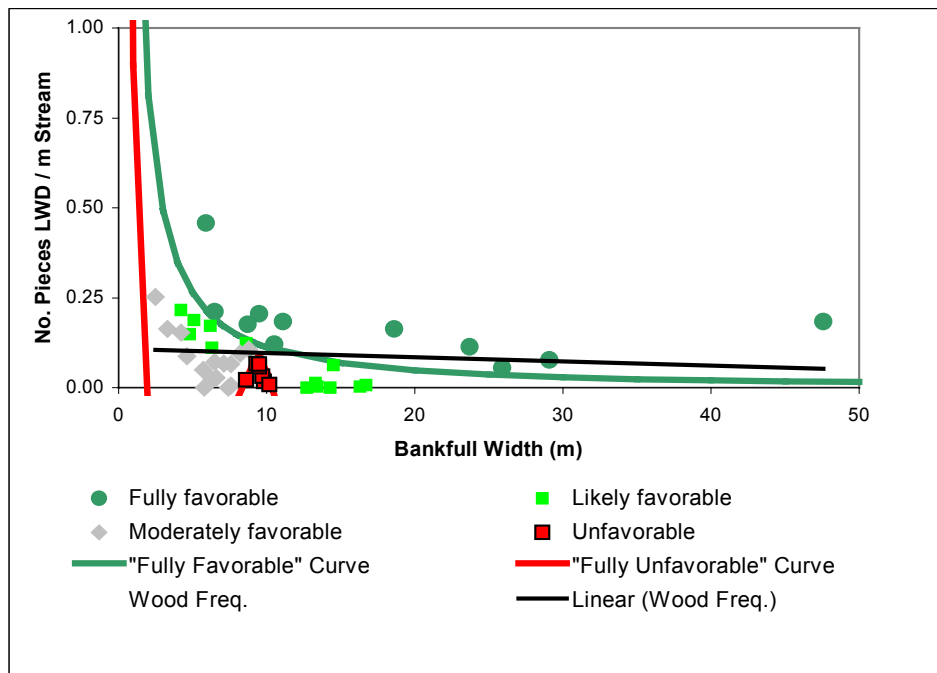
Figure 13. Plot of large woody debris frequency versus bankfull width, color coded by EMDS category, over EMDS evaluation curves which vary as a function of bankfull width. EMDS curves were derived from Bilby and Ward's (1991) data from second growth forests.
