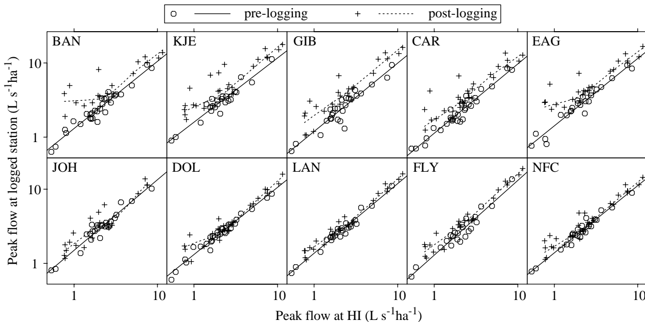
Figure 3 — Relation between peak streamflow in the 10 treated tributaries in the North Fork of Caspar Creek, using the mean of untreated tributaries HEN and IVE (HI) as a control. Pre-logging years began in WY 1986. Post-logging years began in 1990, 1991, or 1992 depending on watershed (see Henry, table 1, these proceedings).
