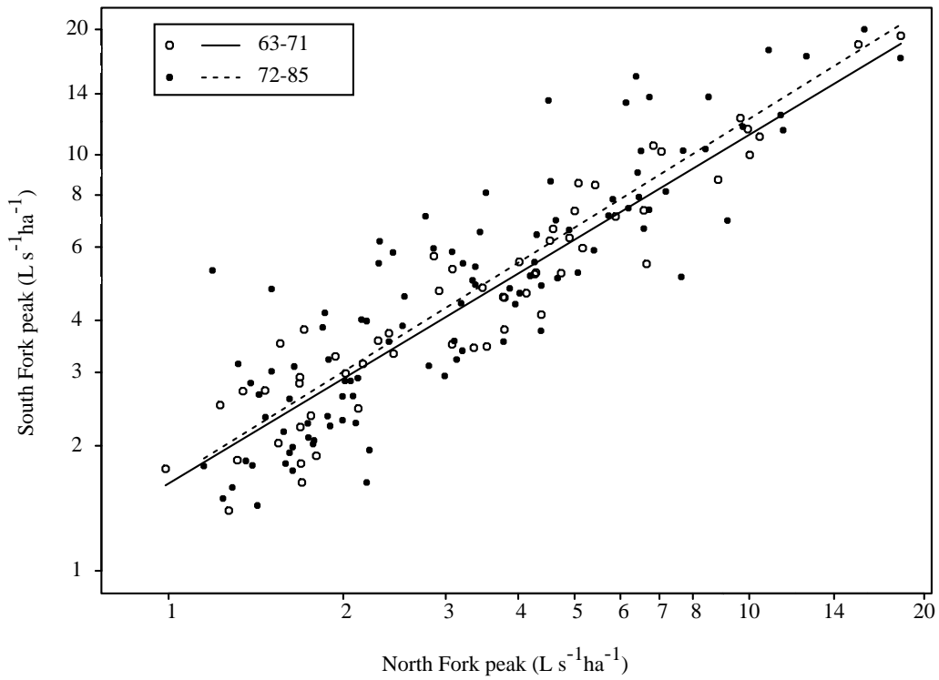
Figure 1 — Relation between peak streamflow in the South Fork of Caspar Creek, using the North Fork as a control. Pre-logging years were 1963-1971, post-logging years were 1972-1985. The two regression lines are not significantly different.
