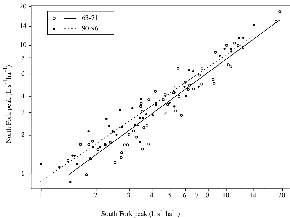
Figure 2 — Relation between peak streamflow in the North Fork of Caspar Creek, using the South Fork as a control. Pre-logging years were 1963-1971, post-logging years were 1990-1996. The two regression lines are not significantly different.
